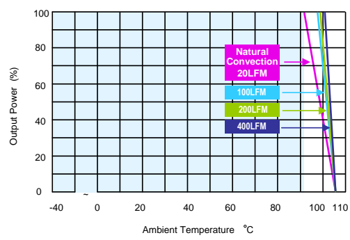
MKZI10-24S24, MKZI10-48D15 Derating Curve with Heatsink
