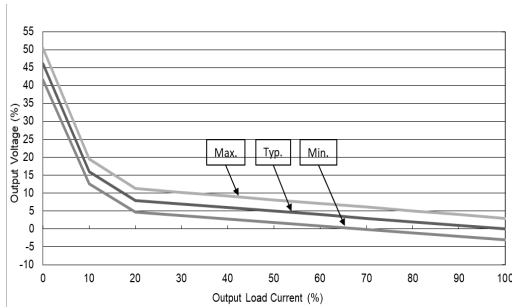
MAU311, MAU312, MAU315, MAU321, MAU322, MAU325 Output Voltage VS Output Load Current
