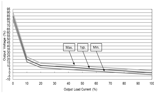
MAU301 & MAU302 Output Voltage VS Output Load Current
