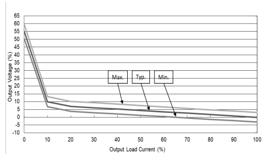
MAU303, MAU304, MAU306, MAU307 Output Voltage VS Output Load Current
