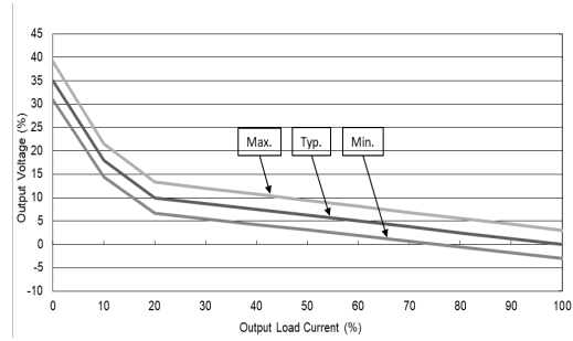
MAU305 Output Voltage VS Output Load Current
