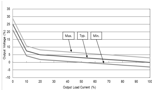
MAU313, MAU314, MAU316, MAU317, MAU323, MAU324, MAU326, MAU327 Output Voltage VS Output Load Current
