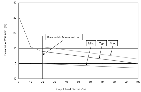
Output Voltage VS Output Load Current For 12V, 15V, ±12V, ±15V Output Models
