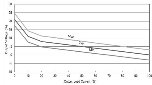
Output Voltage VS Output Load Current For 12V, 15V, ±12V, ±15V Output Models
