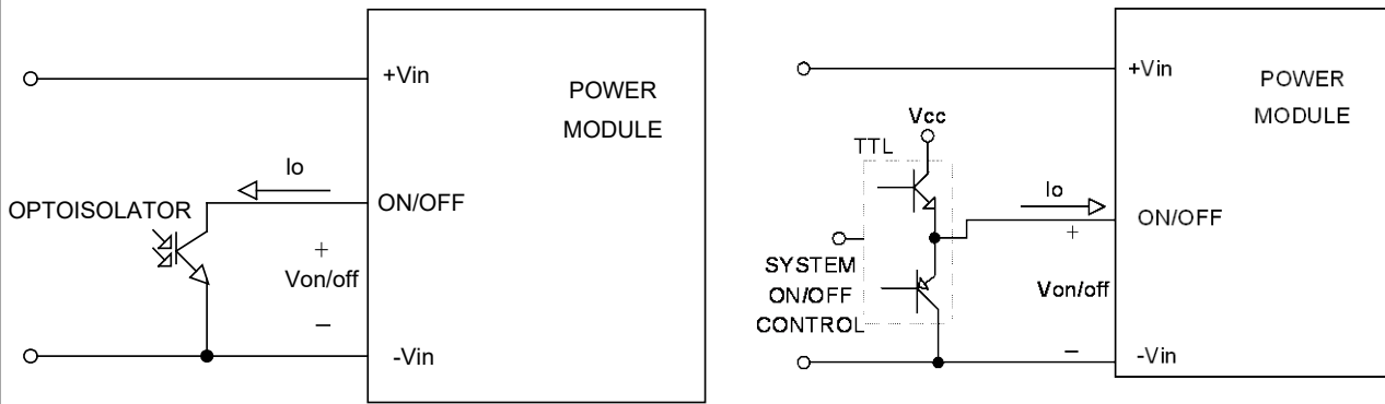
Isolated-Closure Remote ON/OFF
