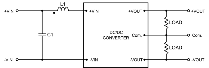
Dual Output
