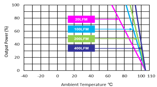
MJWI25-48S033 Derating Curve with Heatsink
