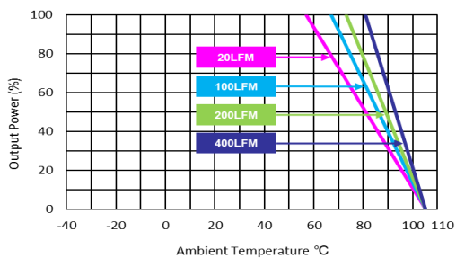
MJWI25-48S033 Derating Curve without Heatsink
