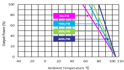
MJWI25-24S15, MJWI25-48S05, MJWI25-48S12, MJWI25-48S15 Derating Curve without Heatsink
