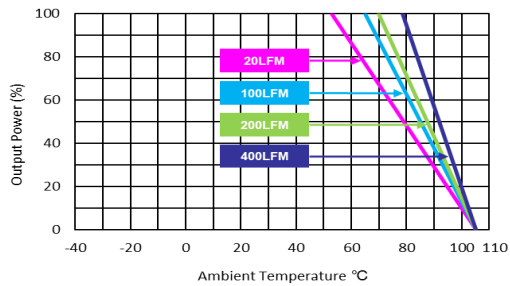
MJWI25-24S033 Derating Curve without Heatsink
