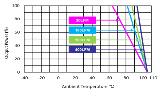
MJWI25-24S15, MJWI25-48S05, MJWI25-48S12, MJWI25-48S15 Derating Curve with Heatsink
