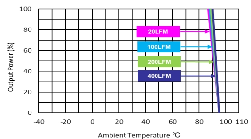
MOWI20-24S051C, MOWI20-48S051C
