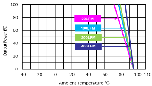
MQWI40-24S48C, MQWI40-48S051C
