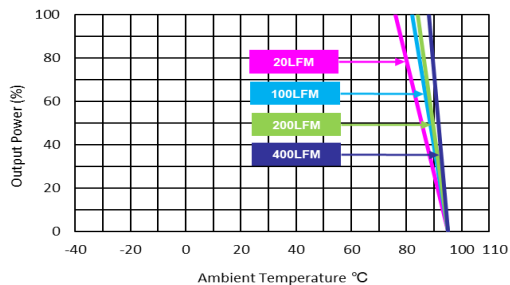
MQWI40-48S12C
